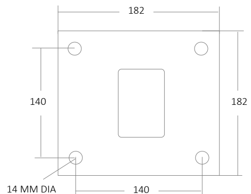
DIMENSIONS AND FASTENER POSITION FOR WALL/ BASE PLATE MOUNT FOR: SER1&2 SEQ1&2/SQ1300/SEW300/SEW600
